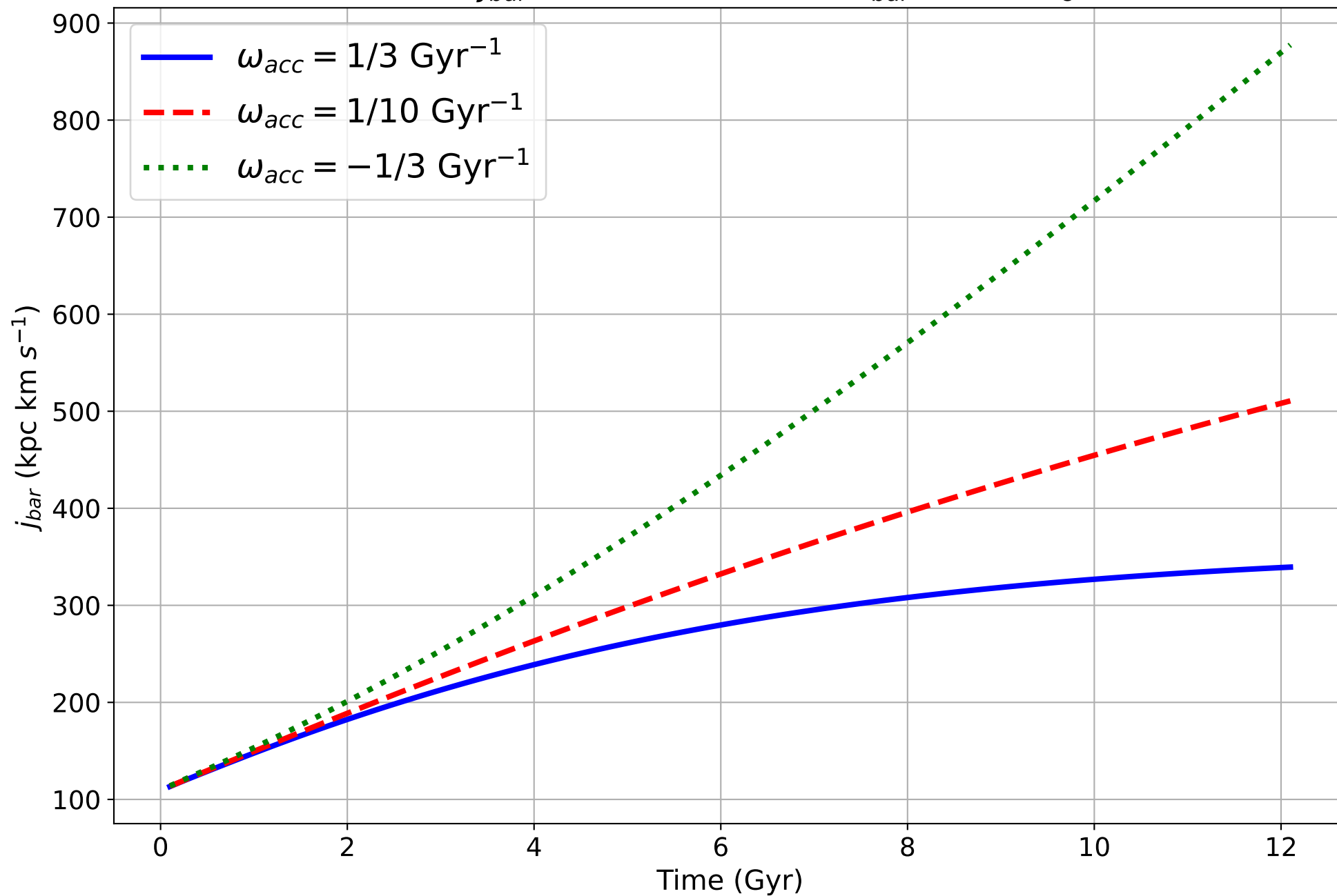
Global j_{bar} vs t (Boissier SFL, M_{bar} = 10^{10} M_{\odot} )
